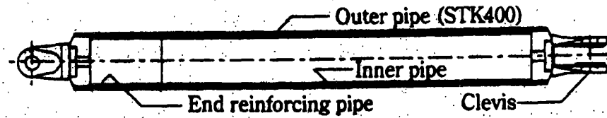
Fig. 12 Outline of double tube bracing
