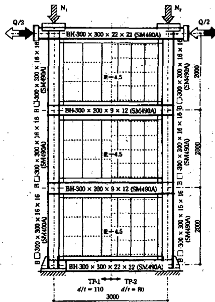
Fig. 9 Three-story frame with low yield stress steel plate walls
