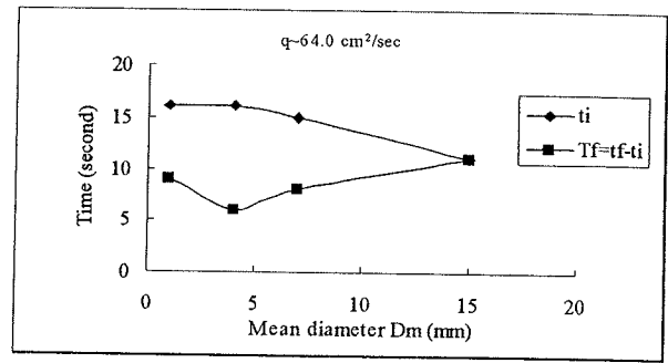
Fig. 4 Mean diameter versus time required for collapse
