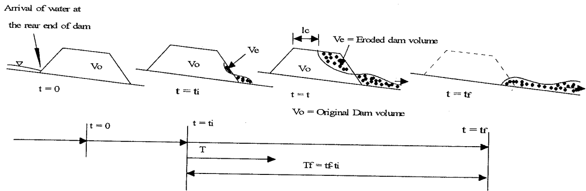
Fig.3 Definition sketch of time, eroded volume and collapse position l_c
