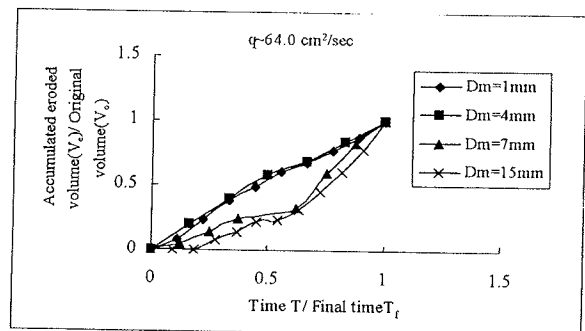
Fig.5 Relationship between non-dimensional eroded volume versus time at approximately same discharge
