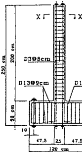
Fig. 3 Test specimens
