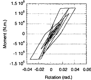
Fig. 6 moment-rotation curve for the bottom of the RC pier
