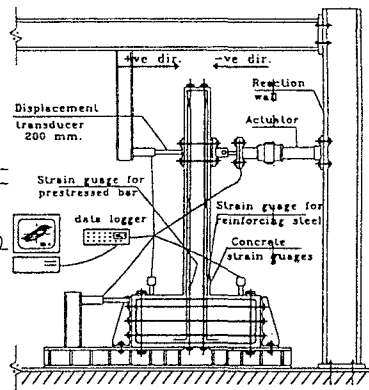
Fig. 4 Loading setup
