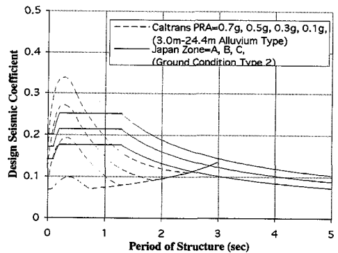
Fig.7 Comparison of design seismic coefficients for a single column bent
