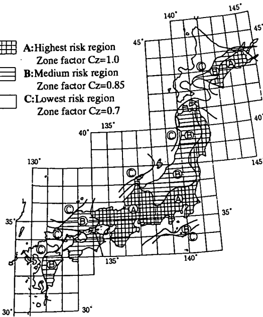
Fig.5 Regional classification of intensity of earthquake motion 19)
