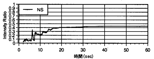
図-21 Arias Intensity 比 (関震協尼崎)
