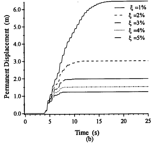
Fig. 8 Acceleration records, and permanent displacement versus time during earthquake for various coefficients of damping, (a) Kushiro earthquake, (b) Kobe earthquake
