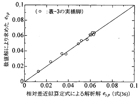
(e) e_{5p}
