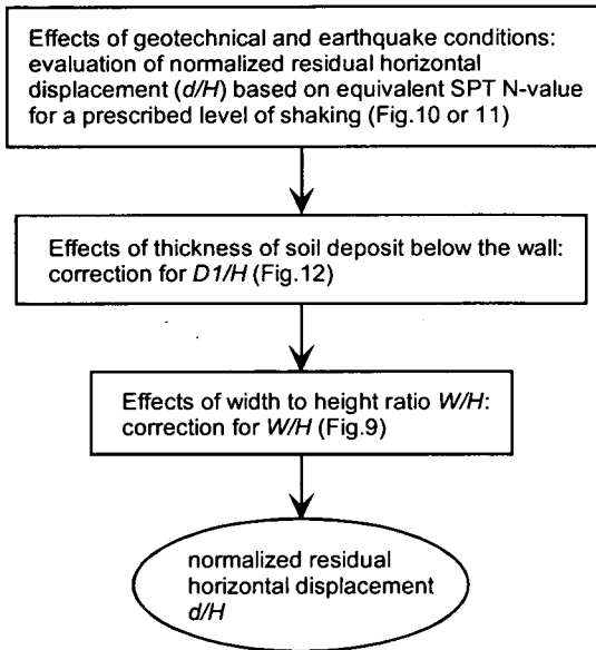
Fig.13 Procedures to evaluate the quay wall displacement
