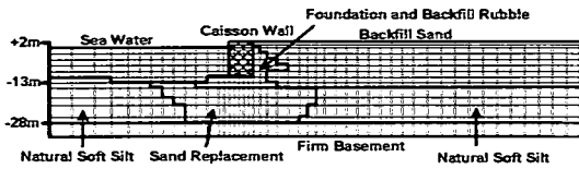
(a) An example of FEM Mesh and Material Configuration
