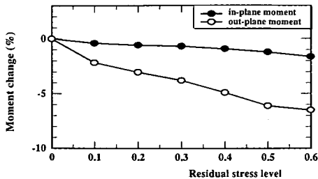
Fig. 16 Moment & residual stress level at tower base
