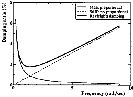
Fig. 2 Damping ratio and frequency relationship
