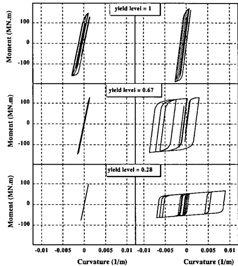
(a) At tower base (b) At horizontal beam end Fig. 20 Moment & curvature relationship
