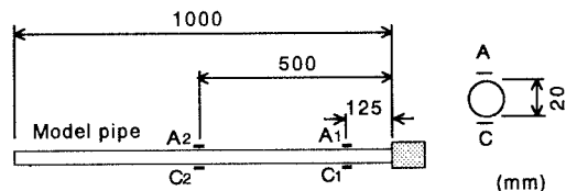
Fig.2 Model pipe and strain gauges.
