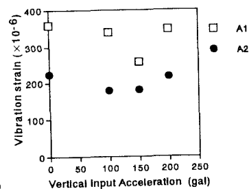
Fig.4 Relationship between vertical input acceleration and vibration strain.
