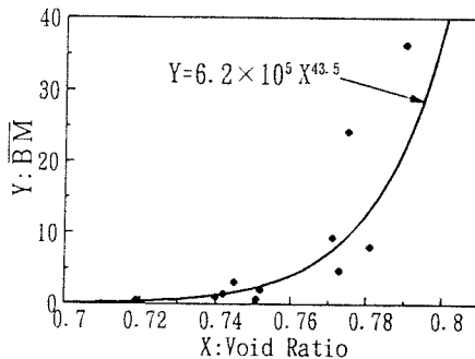
Fig. 6 Collapse Surface on BM-e Plane
