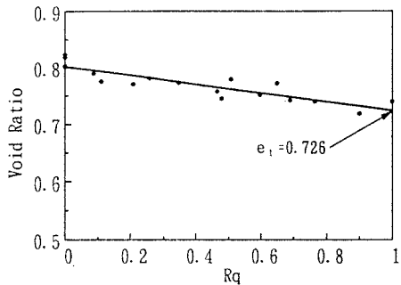
Fig. 4 Relationships between Rq and Void Ratio
