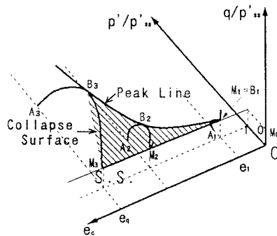
Fig. 5 Collapse Surface on e-p'/p'_{ss}-q/p'_{ss} Space
