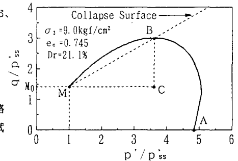
Fig. 3 Normalized Stress Path
