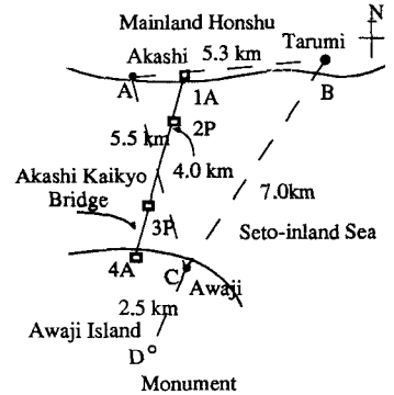
Fig.1 Location of Akashi Kaikyo Bridge and array observation system.
