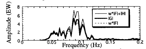
Fig.4.1 Fourier amplitude spectra of NO.55 at Akashi Station.
