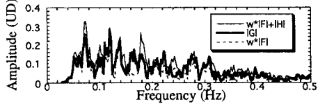
Fig.4.2 Fourier amplitude spectra of NO.69 at Monument Station.
