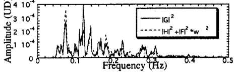
Fig.3.2 Power spectra of observed wave and remainder wave + beam*weight**2 at Monument Station (NO.69).
