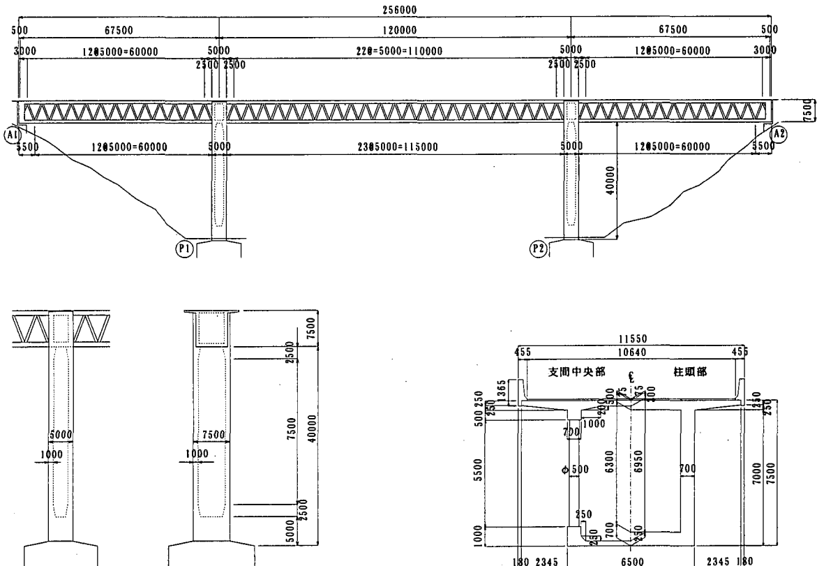
図-1 検討対象橋梁
