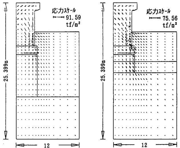
(a) Model-1N
