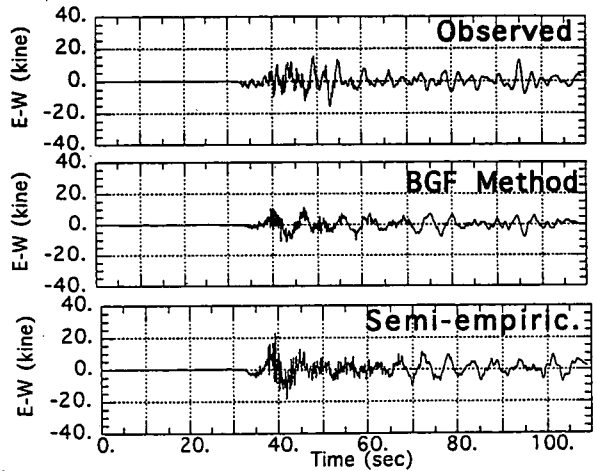
Fig.6: Velocity time histories of Observed and Synthetic signals of the mainshock at Sakai Station. Component E-W.
