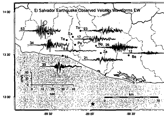
Figure 2. Spatial Distribution of the recorded velocities waveforms EW and NS components, during the January 13/2001 El Salvador earthquake. The PGV values at each station are shown. The CIG epicenter is shown by a star.
