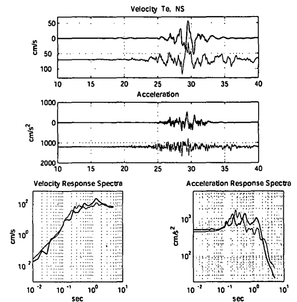
Figure 5. Comparison between the simulated (thick line) and observed NS component (velocity and acceleration waveforms and response spectra) at the Te station (Hospital San Rafael, Santa Tecla) during the January 13, 2001 El Salvador earthquake. The waveforms are bandpassed filtered between 0.1 and 10 Hz.
