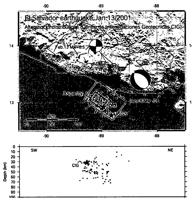
Figure 1. USGS focal mechanism solutions and CIG aftershocks distribution of the El Salvador January 13, 2001 earthquake (dark gray) The approximate rupture area corresponding to the USGS fault plane solution No. 2 is shown by a rectangle. The CIG and USGS epicenter are shown by a star. The asperity rupture model determined by this study is shown by a thick rectangle. Aftershocks projection perpendicular to the USGS fault plane solution No. 2 is shown (Lower panel).
