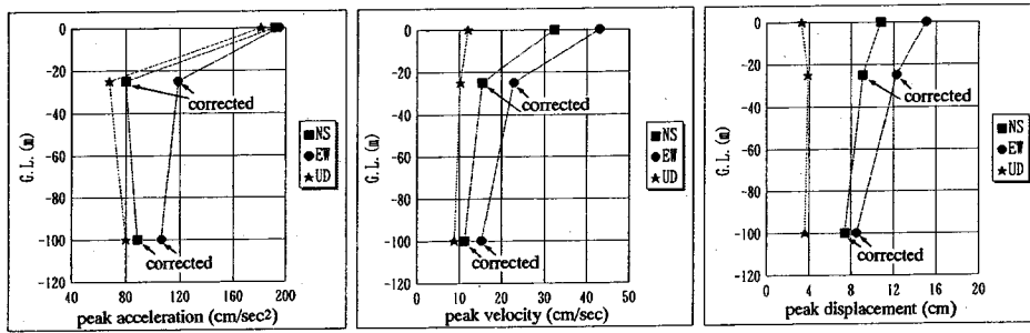
Fig. 13 Distribution of Peak Ground Motions (Takasago Power Station, Kansai Electric Power Company).
