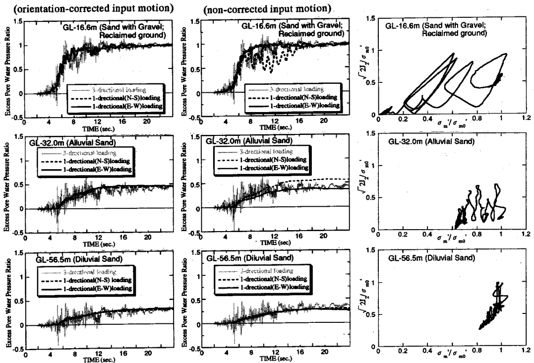
Fig. 16 Time Histories of Excess Pore Water Pressure Ratio and Effective Stress Path in Numerical Analysis.
