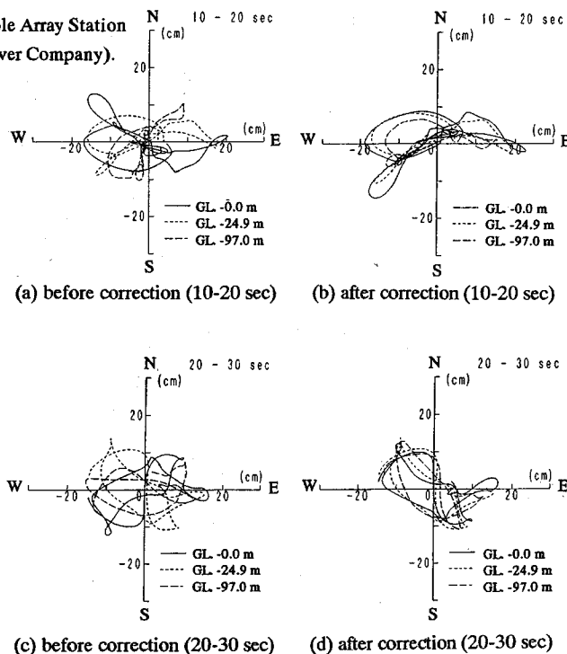
Fig.5 Displacement Orbits (Technical Research Center, Kansai Electric Power Company).
