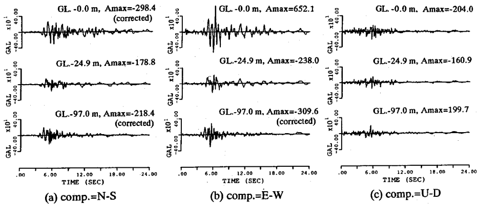
Fig.6 Acceleration Time Histories (Technical Research Center, Kansai Electric Power Company).
