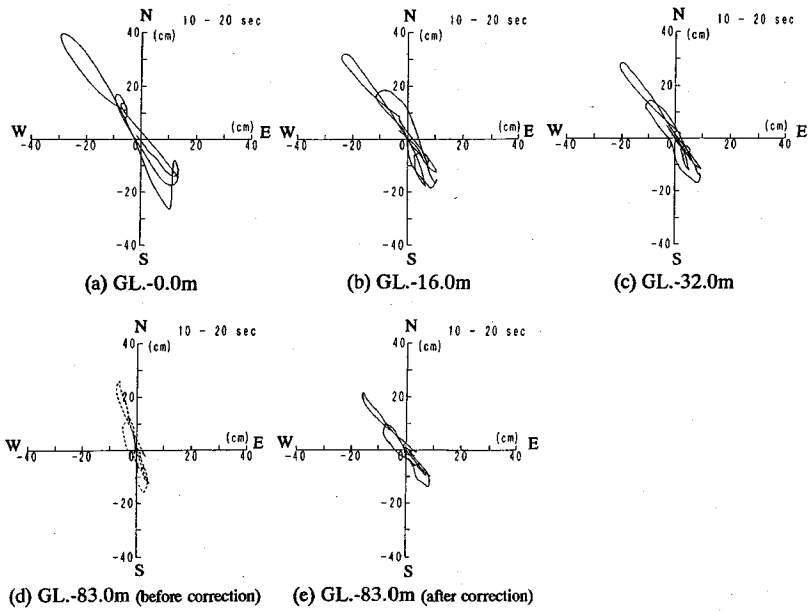
Fig.2 Displacement orbits at various depths (Port Island, Kobe City, 10-20 sec, 0.15-20.0 Hz).
