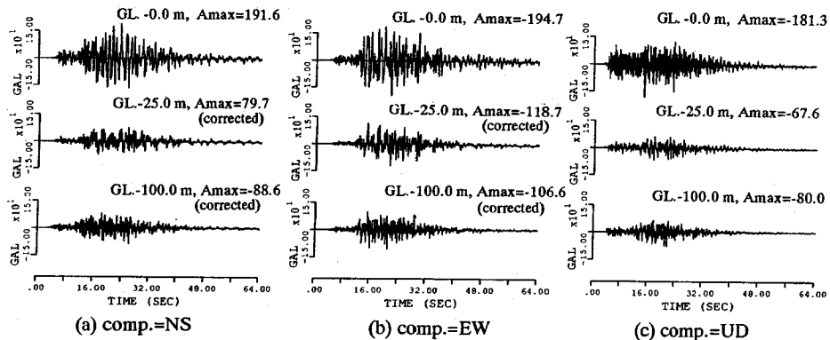
Fig. 12 Acceleration Time Histories (Takasago Power Station, Kansai Electric Power Company).
