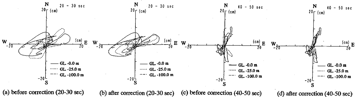
Fig. 11 Displacement Orbits (Takasago Power Station, Kansai Electric Power Company).
