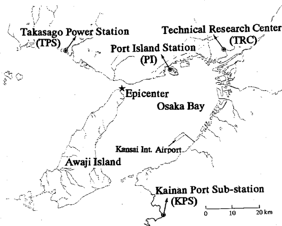
Fig.1 Location of Borehole Array Observation Stations.
