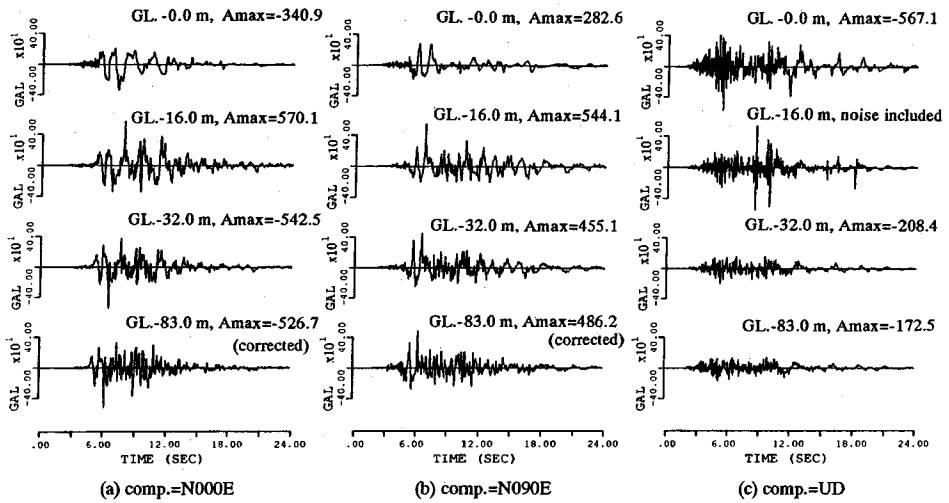
Fig.3 Acceleration Time Histories (Port Island, Kobe City Development Bureau).
