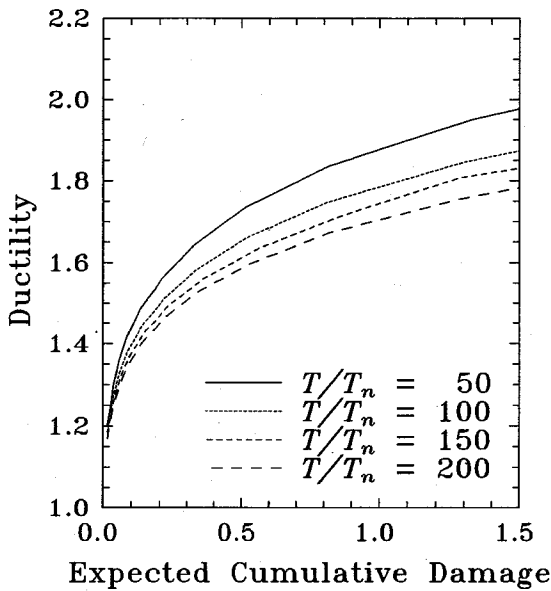
Fig.3 Variation in Ductility, \mu with Expected Cumulative Damage, E(D) for Concrete.
