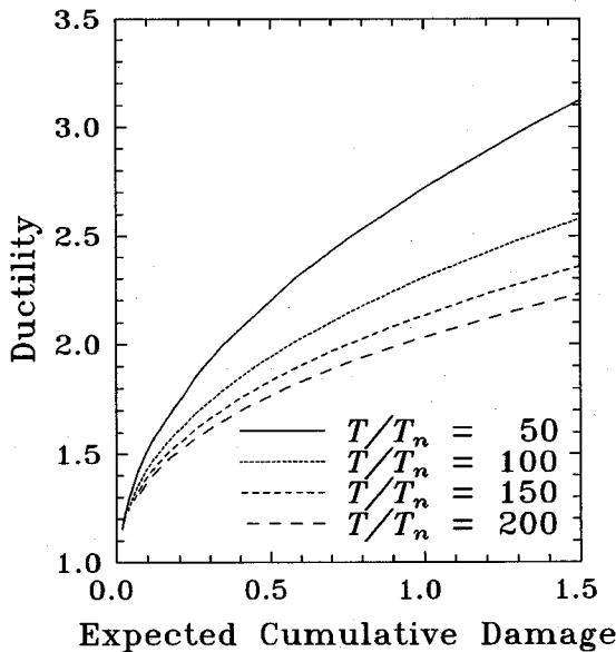
Fig.4 Variation in Ductility, \mu with Expected Cumulative Damage, E(D) for Steel.
