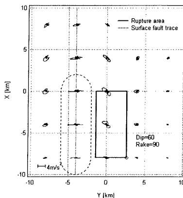
Fig.4 Acceleration trajectories for the mechanism of (dip= 60^\circ , rake= 90^\circ ).
