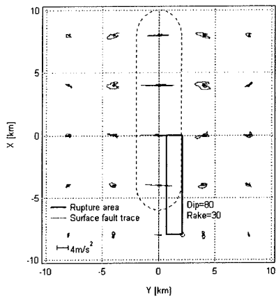
Fig.5 Acceleration trajectories for the mechanism of (dip=80°, rake=30°).
