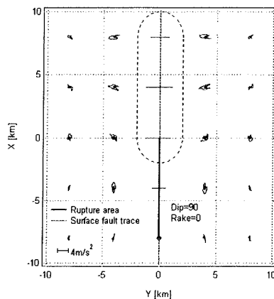
Fig.3 Acceleration trajectories for the mechanism of (dip= 90^\circ , rake= 0^\circ ).
